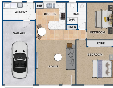
FLOOR PLAN
